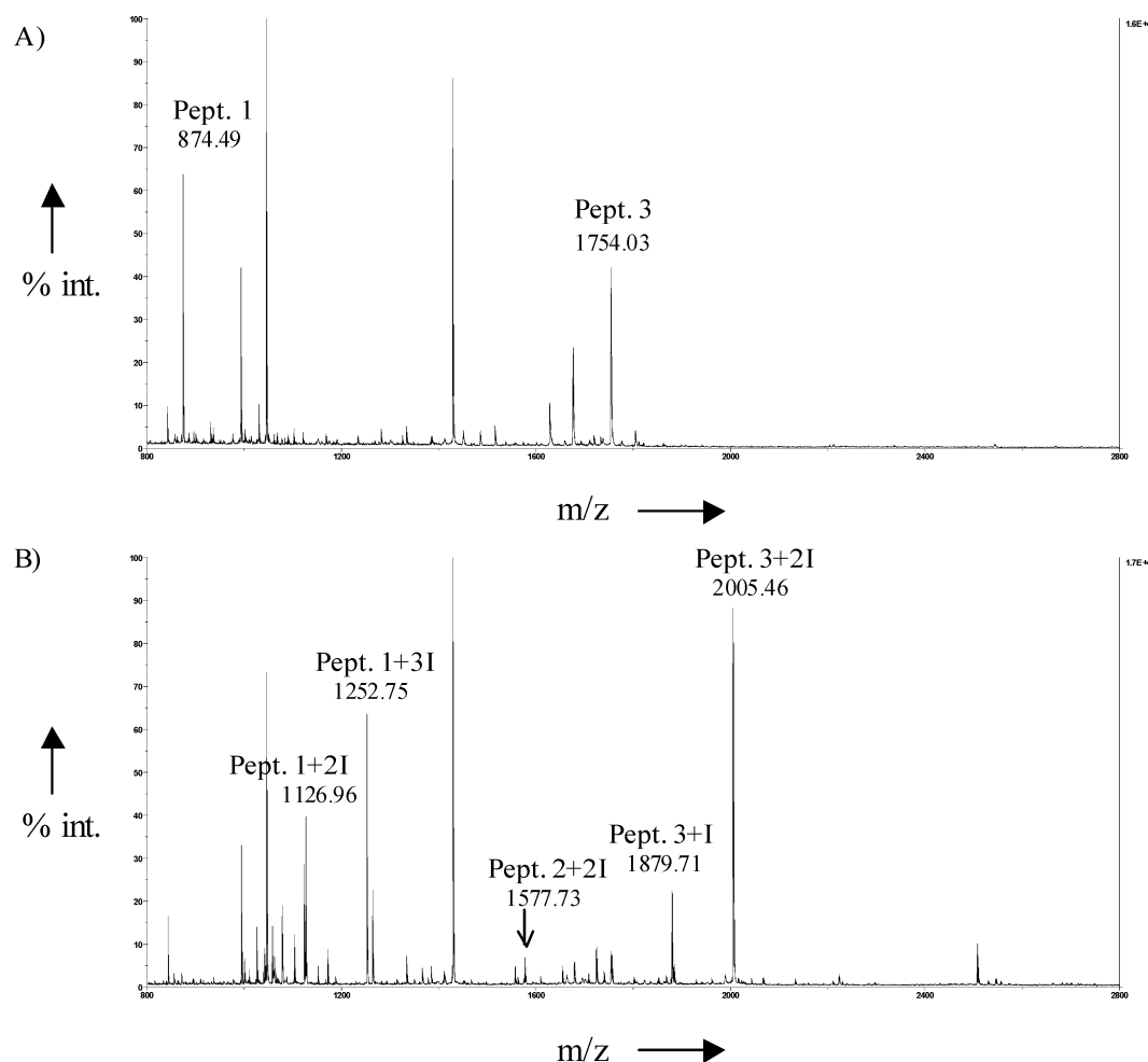
FIGURE 2: MALDI-TOF-MS of tryptic digestion of (A) lysozyme and (B) iodinated lysozyme with 18.7 equiv of IPy 2 BF 4 . Peptides 1 , 2 , and 3 are represented as Tyr- and His-containing fragments. (See the description in the text and in the Supporting Information.)
