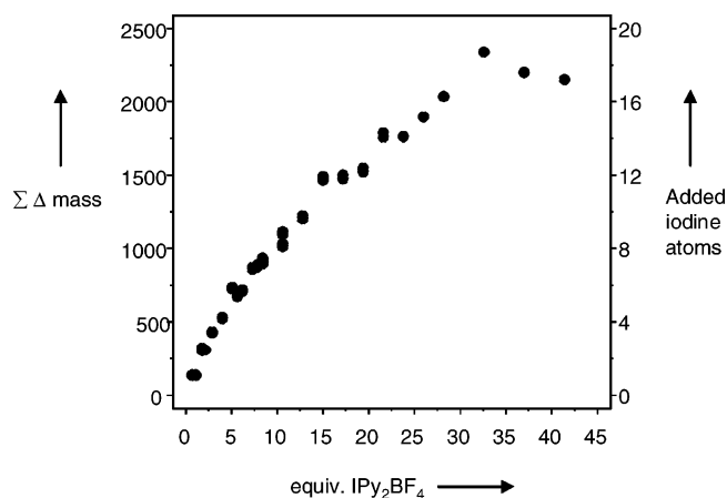
FIGURE 4: Changes in the mass and number of incorporated iodine atoms of 1,3-1,4- \beta -D-4-glucanohydrolase at different stoichiometries of IPy 2 BF 4 . Experimental conditions are described in the text.
