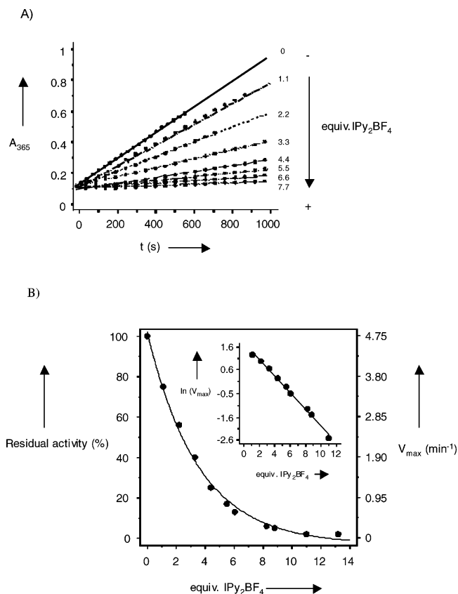
FIGURE 3: Activity of 1,3-1,4- \beta -D-glucanohydrolase after treatment with different concentrations of IPy 2 BF 4 . Enzymatic activity was measured at 365 nm by incubating the chemically modified enzyme with a constant concentration of substrate, Glc \beta 1,4Glc \beta 1,3Glc \beta -MU (2.4 mM) at 30 °C in a citrate/phosphate buffer (6.5 mM citric acid, 87 mM Na 2 HPO 4 , pH 7.2) and CaCl 2 (0.1 mM). (A) Time-course monitoring of the release of 4-methylumbelliferone (MU) from the substrate at different IPy 2 BF 4 concentrations. (B) Residual activity vs IPy 2 BF 4 concentration.
